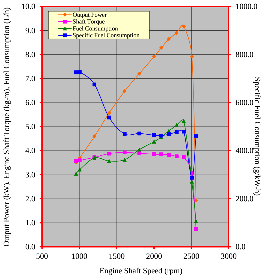
Figure 3. Performance characteristic curves of the KUVICO KV125-2 diesel engine
