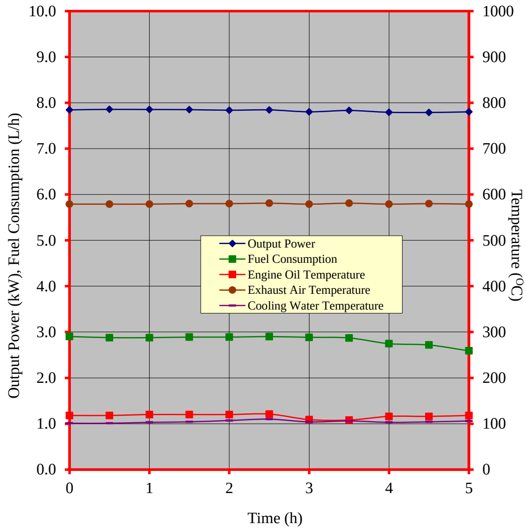
Figure 4. Performance characteristic curves during the continuous running test of the KUVICO KV125-2 diesel engine
